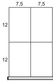
L_BG-A0102 4 compartments
