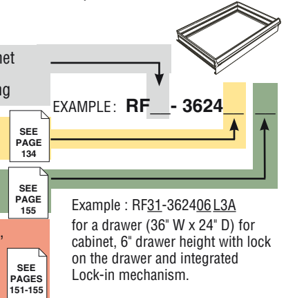
Drawer dimensions
