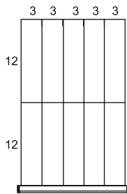
L_BG-A0405 10 compartments
