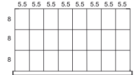
R_HG-A0716 24 compartments
