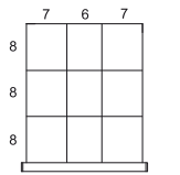
R_CG-A0206 9 compartments
